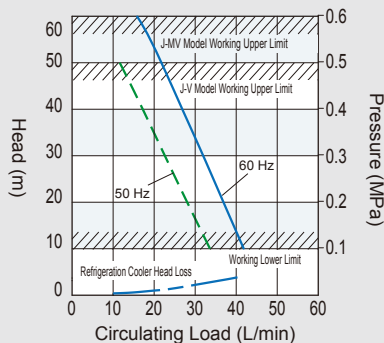
High Head / High Flow-Rate Pump For RKS402/75□J-MV* 1 For RKS753J-V* 2
