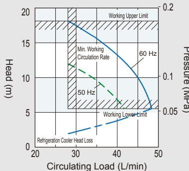
Pump w/Copper-Less Spec. Wetted Parts For RKS40□/75□J-MV* 1 For RKS753J-V* 2
