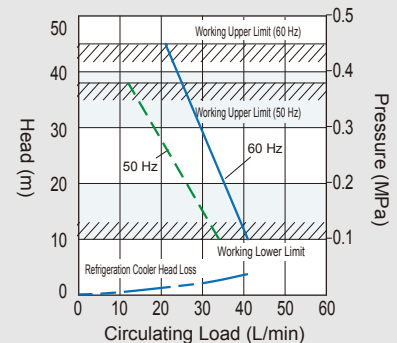
Pump w/Copper-Less Spec. Wetted Parts For RKS150□J-MV* 1 For RKS1503J-V* 2
