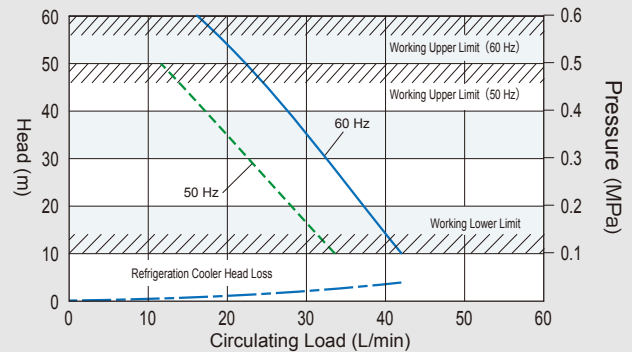
RKS1502/1503J-MV* 1 RKS1503J-V* 2 (Working Upper Limit: 50 m)
